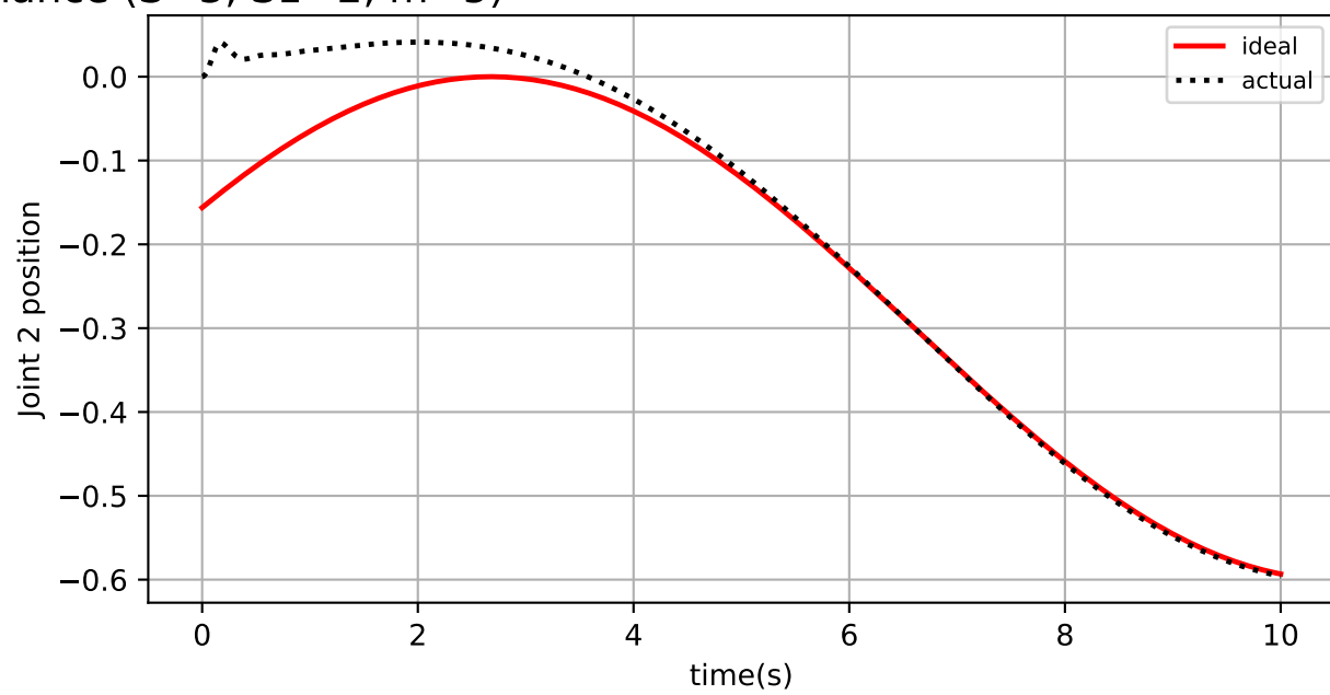
Position Tracking Performance (S=3, S1=2, m=5)
